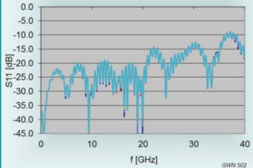
S11 (f)
