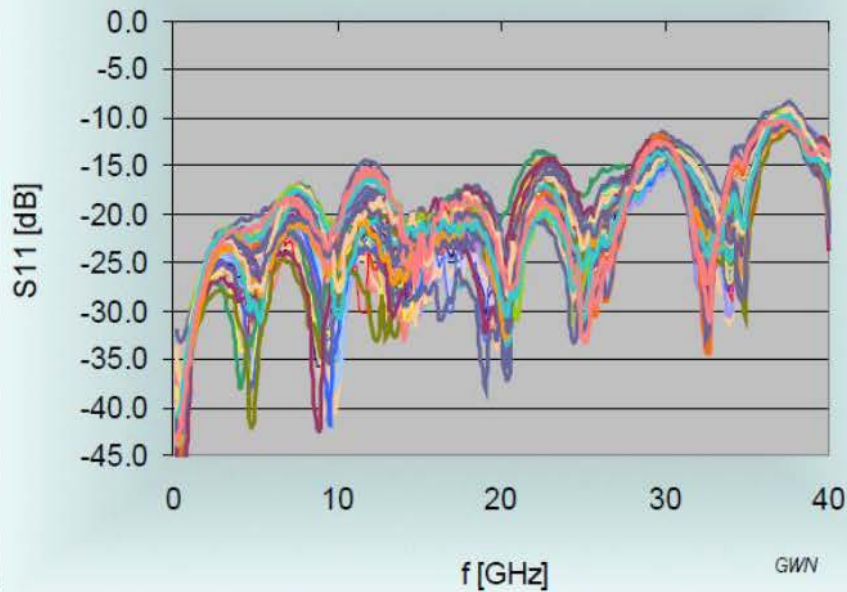
S11 (f)
